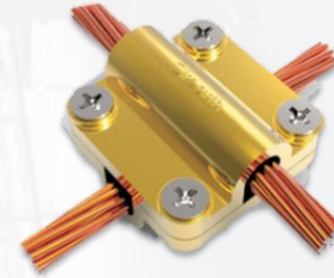
4 way connection
