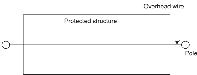
FIGURE A.4.6.5.2(a) Single Overhead Wire Lightning Protection System.
