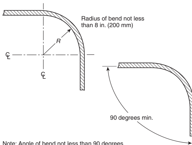
FIGURE 4.9.5 Conductor Bends.
