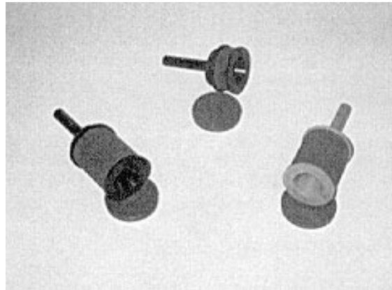
Figure 5-5—Flame arrester vents with dust covers
